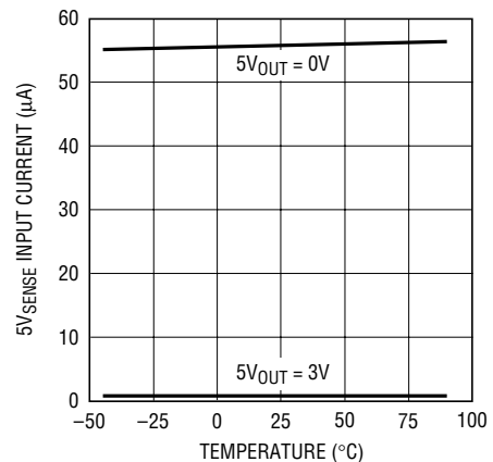
5V SENSE Input Current vs Temperature
