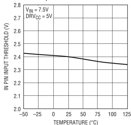
IN High Threshold Voltage vs Temperature
