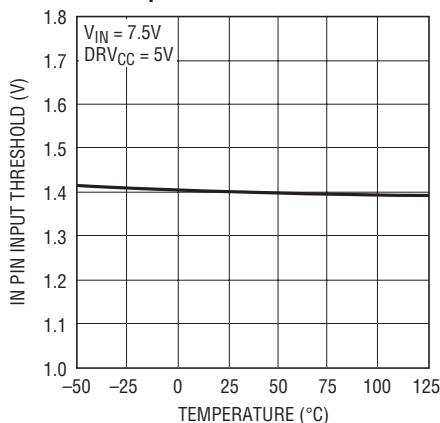
IN Low Threshold Voltage vs Temperature
