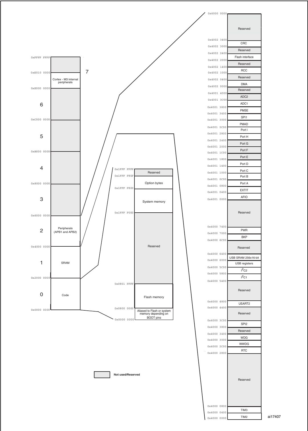
Figure 3. Memory map
