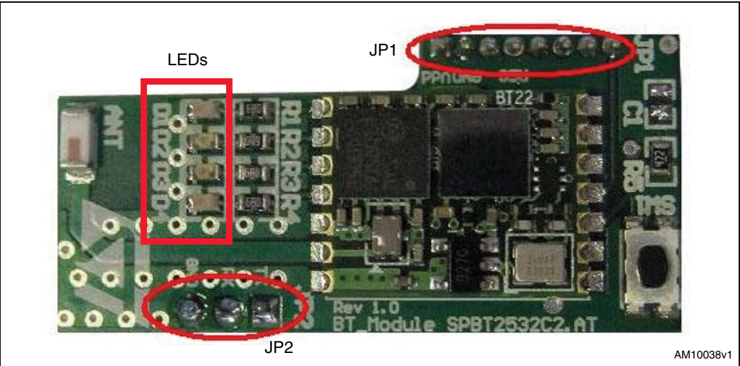
Figure 4. STEVAL-MKI115V1 connectors
