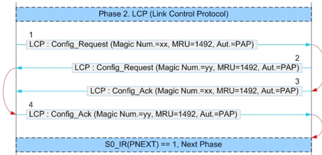
Figure 4. PPP LCP Configuration Process
