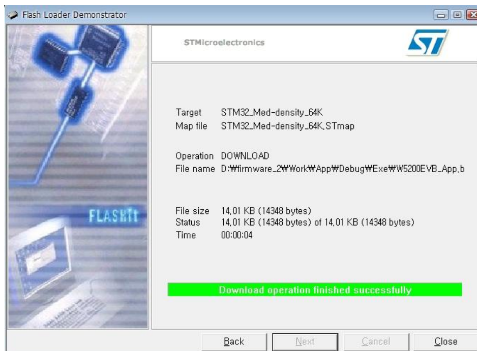
Fig. 4.8 Download Completion
