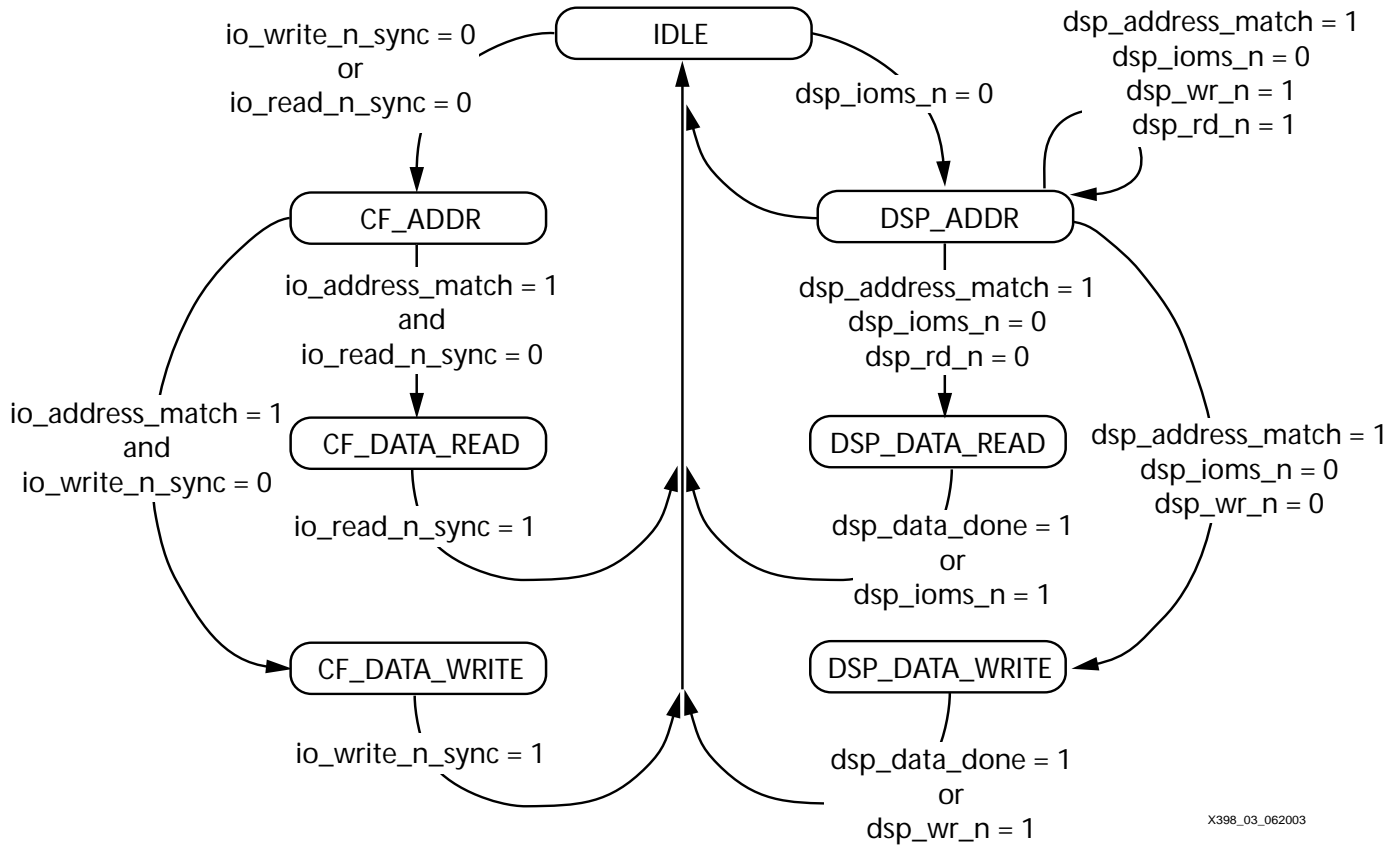
Figure 3: I/O Space State Machine
