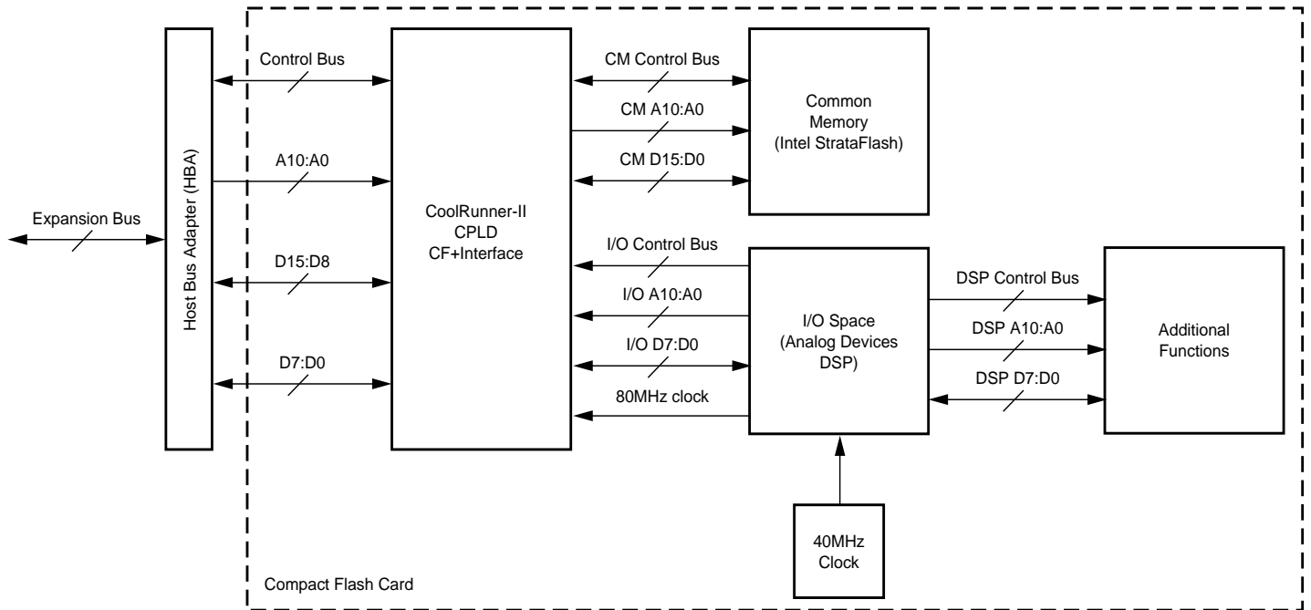
Figure 1: CompactFlash Card General Block Diagram
